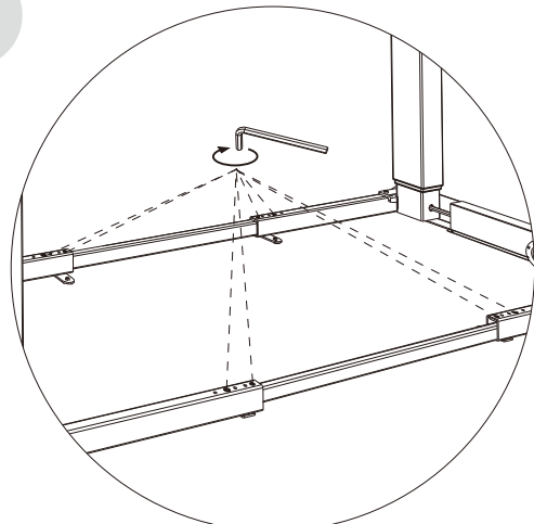
Pre-tighten screws
